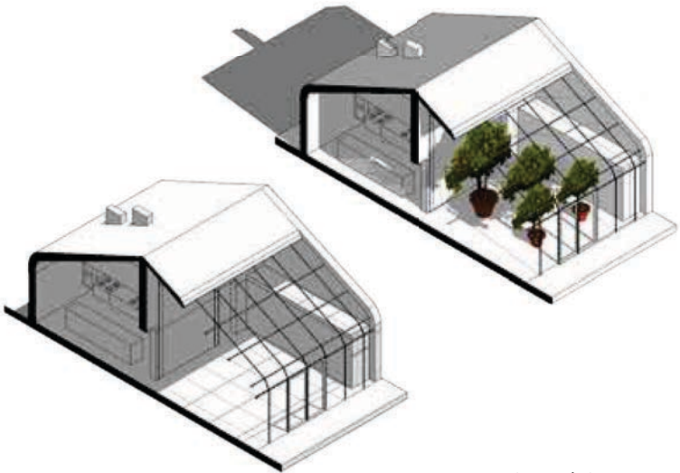
winter solstice
