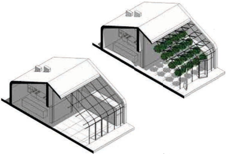
summer solstice
